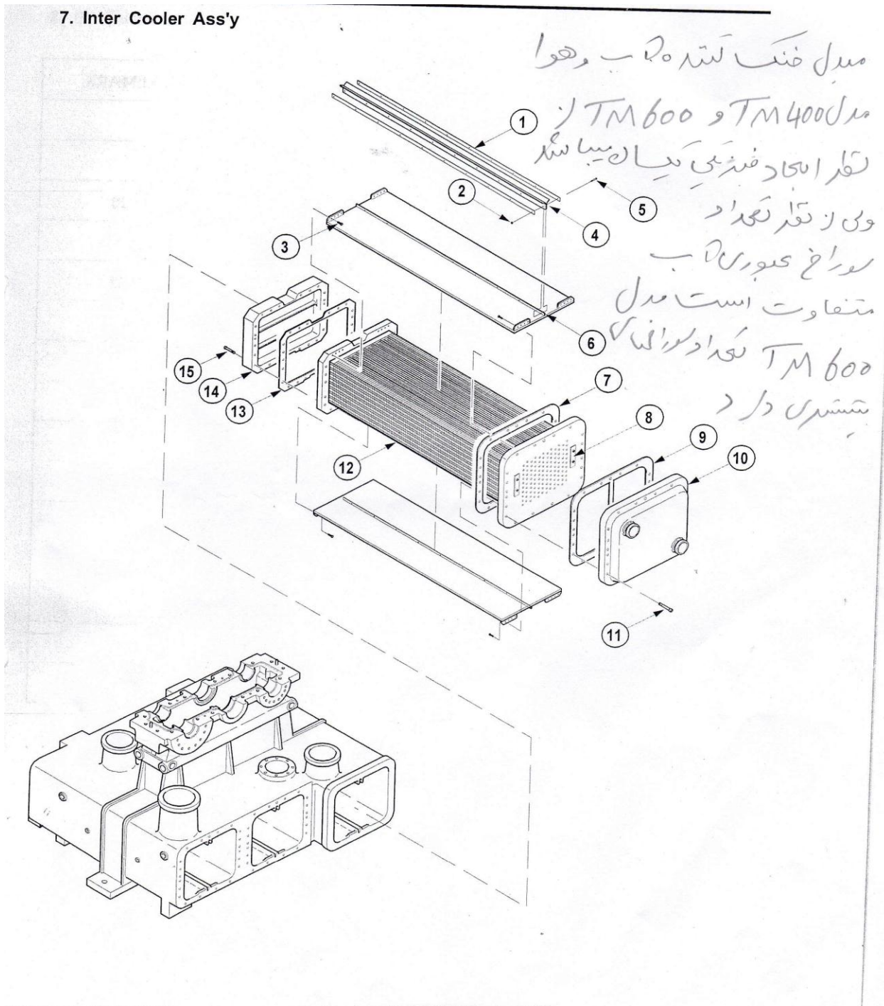
FIG.7. INTER COOLER Assembly
