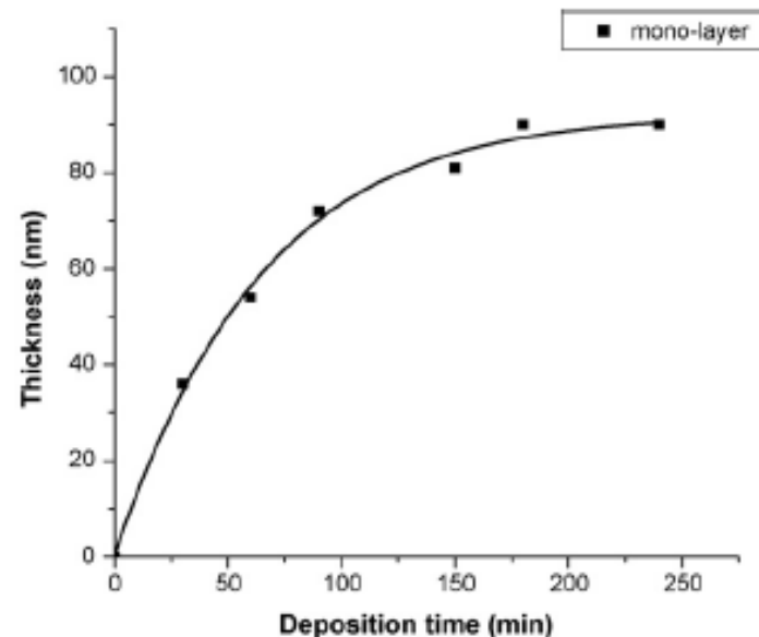
Fig. 2. Thickness as a function of deposition time for monolayer ZnS films deposited under standard conditions.
